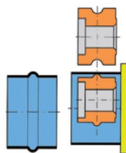
56 Beading rolls
