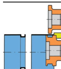
SKS Box Beading rolls
